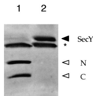
Fig. 3. OmpP-dependent SecY cleavage. Plasmid pCM131 ( ompP ; lane 1) or plasmid pSTV29 (vector; lane 2) was introduced into strain AD202. Resulting transformants were grown at 37°C in L medium containing 0.2% glucose and 10 µg/ml of chloramphenicol and cell lysates were prepared. They were treated with 1.0% Triton X-100 on ice for 10 h, and subjected to SDS-PAGE. The SecY immunoblot was visualized using a LAS-1000 luminescence imager.
